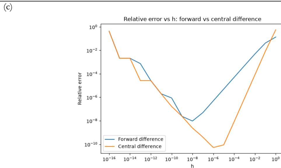
Figure 6: log-log plot to compare the relative error vs h for forward difference and central difference calculations.
