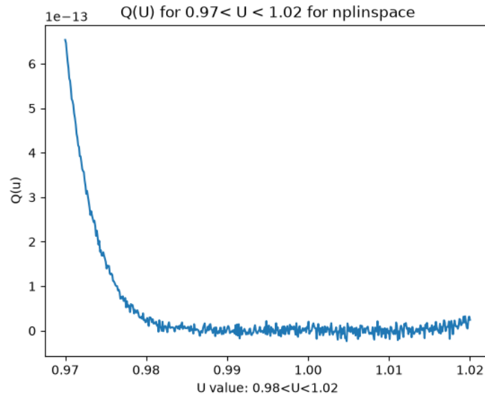
Figure 4: Q(u) = (1-u)^8 , evaluated in its expanded form (formula 6) from for 500 evenly spaced points 0.97 < u < 1.02 . [np.linspace]
