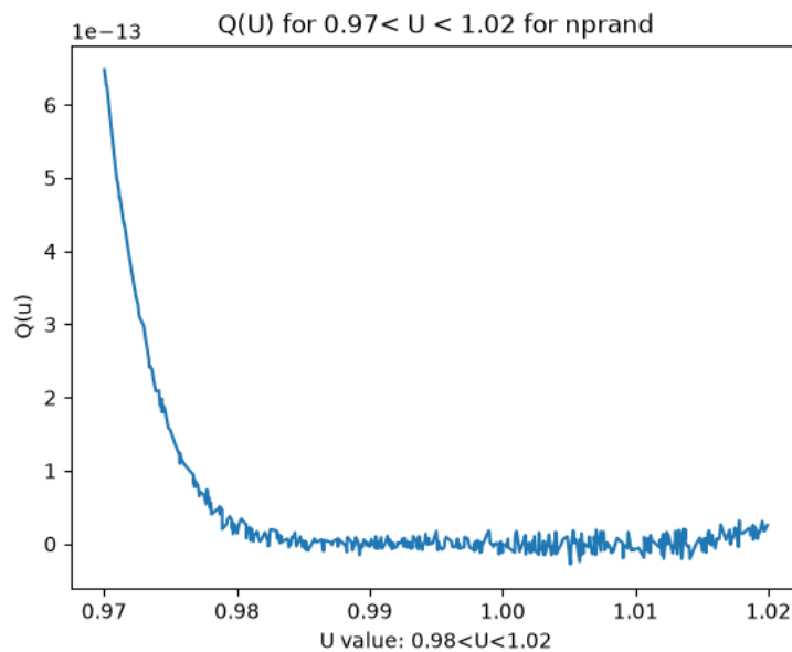
Figure 2: Q(u) = (1-u)^8 , evaluated in its expanded form (formula 6) from for 500 evenly spaced points 0.97 < u < 1.02 . [np.rand]
