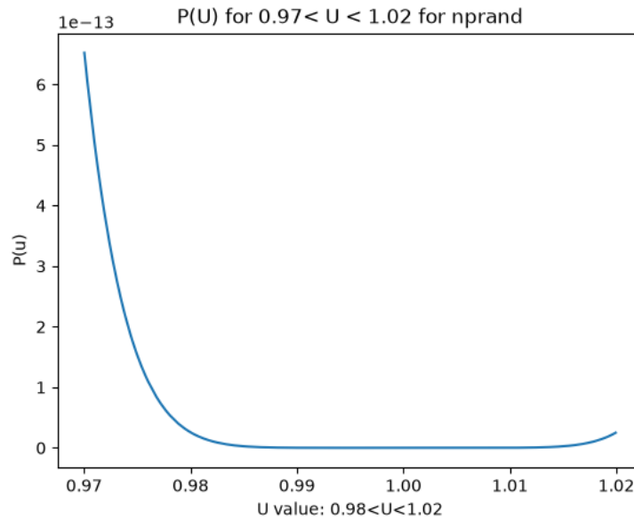
Figure 1: P(u) = (1-u)^8 , evaluated in its factored form for 500 evenly spaced points 0.97 < u < 1.02 . [nprnad]
