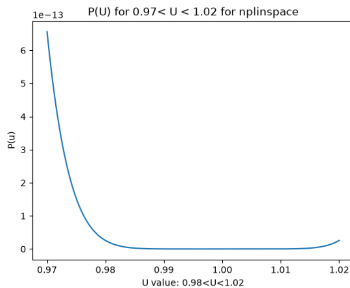
Figure 3: P(u) = (1-u)^8 evaluated in its factored form for 500 evenly spaced points 0.97 < u < 1.02 . [nplinspace]]
